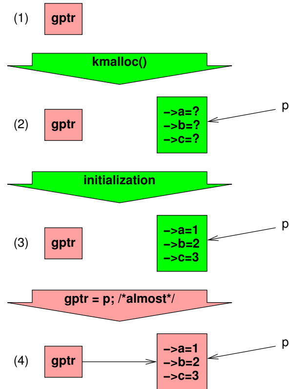
Figure 8.10: Insertion With Concurrent Readers
